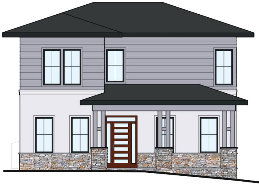
SOUTH ELEVATION
